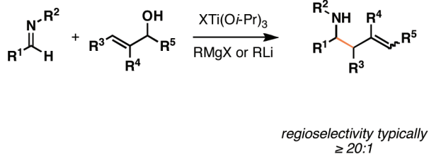
FIGURE 3. Homoallylic amines by Ti-alkoxide-mediated reductive cross-coupling.
