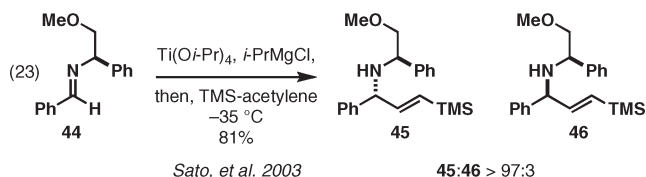
FIGURE 13. Use of a phenylglycine auxiliary in azametallacyclopropane-based coupling reactions.
