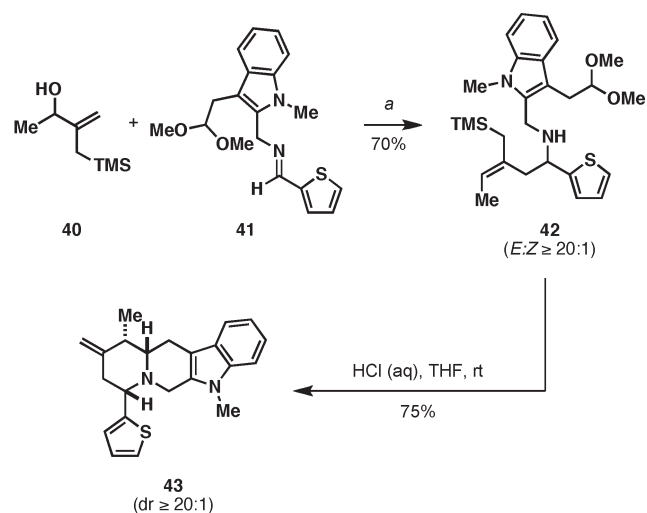
FIGURE 10. Convergent synthesis of complex heterocycles via Ti-mediated coupling of allylic alcohols with imines.
