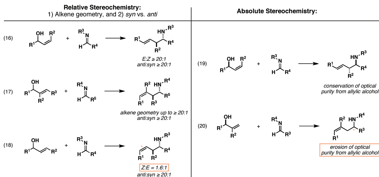
FIGURE 11. Summary of stereochemical observations.
