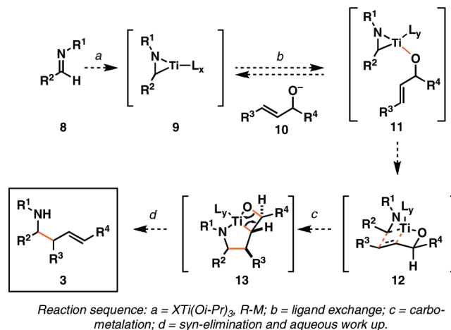
FIGURE 4. General strategy for Ti-alkoxide-mediated coupling of allylic alcohols with imines.
