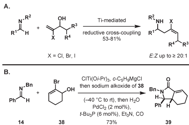
FIGURE 9. One-pot annulation for the synthesis of stereodefined exoalkylidene \gamma -lactams.
